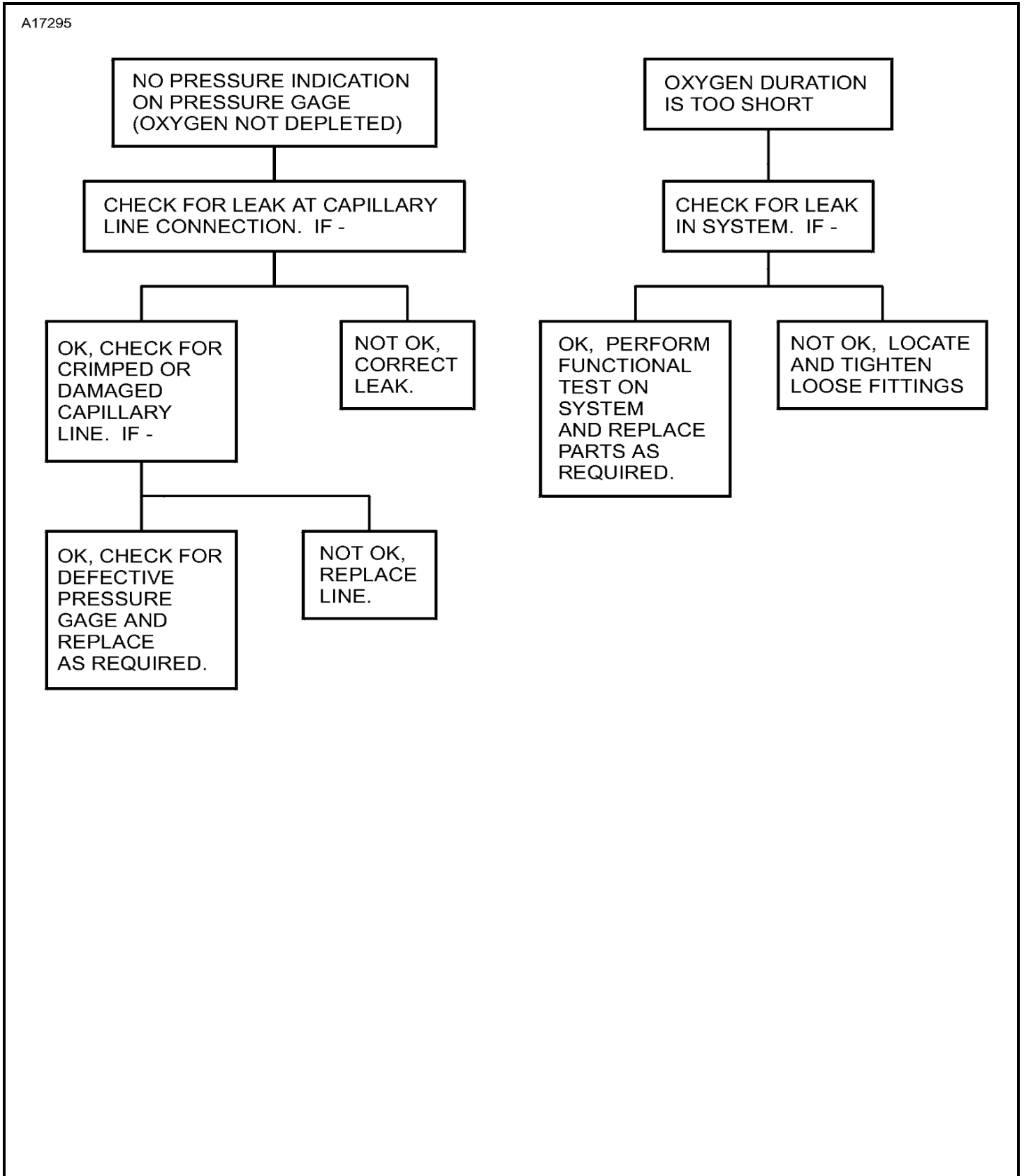
Figure 101 : Sheet 1 : Oxygen System Troubleshooting Chart
