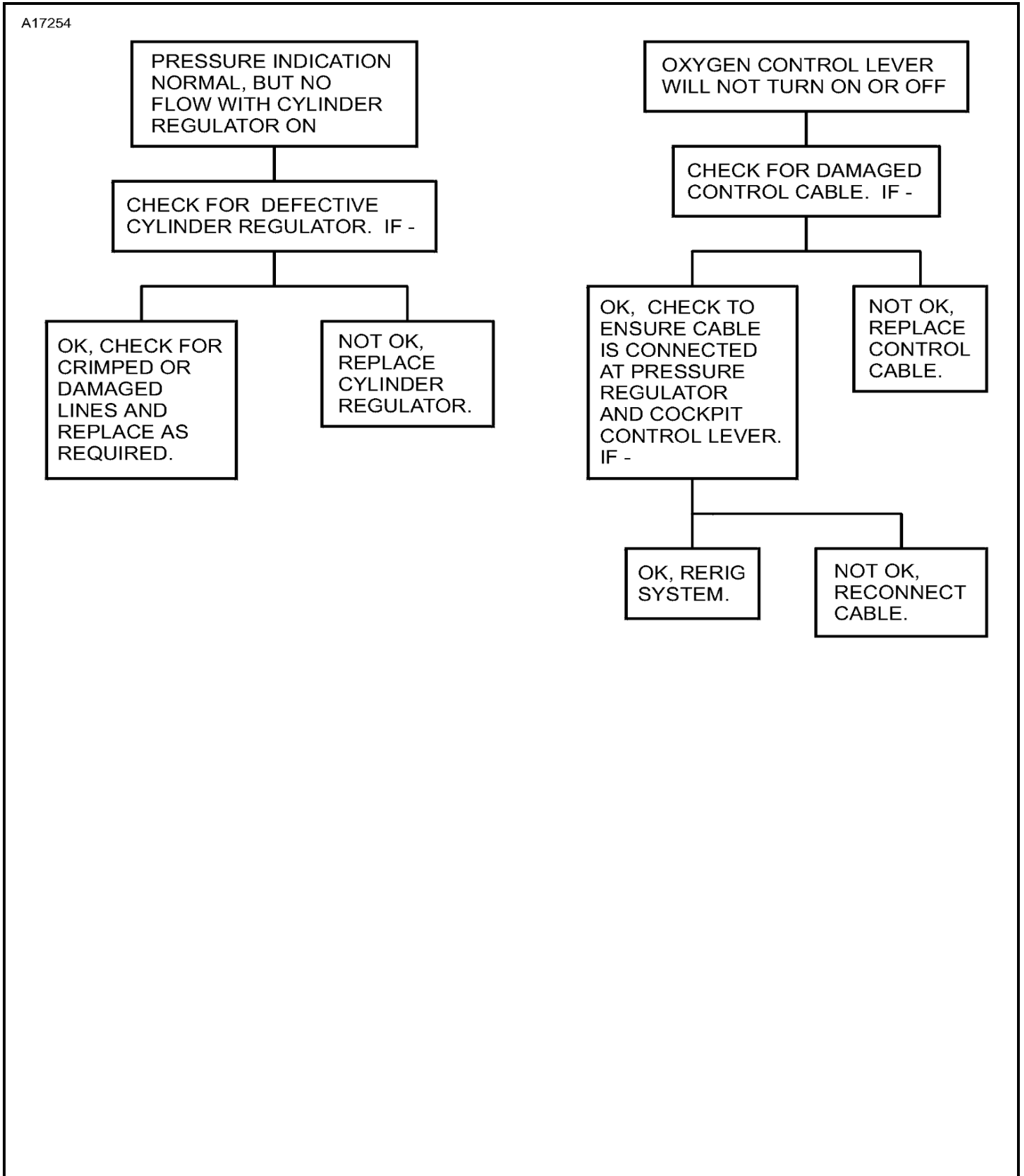
Figure 101 : Sheet 2 : Oxygen System Troubleshooting Chart
